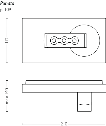
571603LI class I, IP20, SELV H140mm L210mm W112mm
