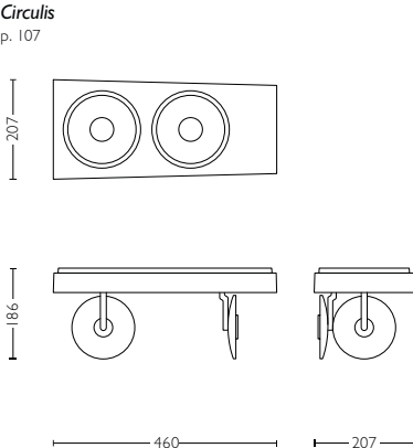
579373116 class I, IP20, SELV H50mm L460mm W207mm
