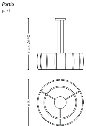
4025232LI class I, IP20, 230V H2640mm L610mm W610mm
