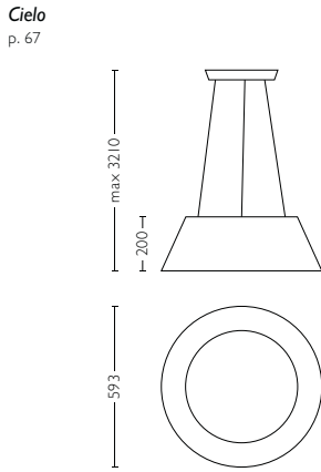
4055030LI class II, IP20, 230V H3210mm L593mm W593mm
