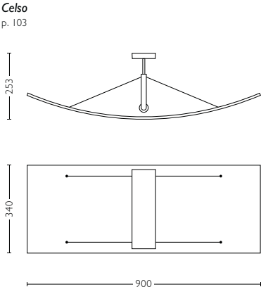
4022117LI class I, IP20, 230V H253mm L900mm W340mm
