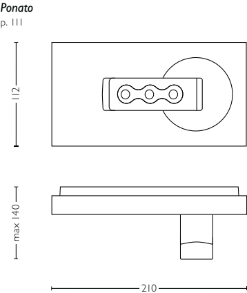
5716013LI class I, IP20, SELV H140mm L210mm W112mm
