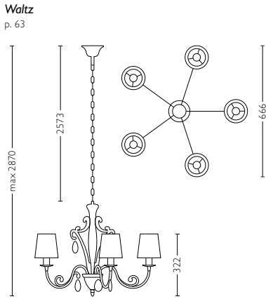
3668031LI class I, IP20, 230V H2870mm L666mm W666mm
