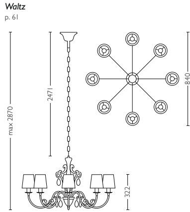
3668130LI class I, IP20, 230V H2870mm L840mm W840mm
