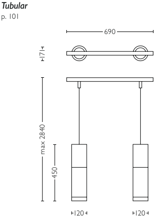
402161LI class I, IP20, 230V H2840mm L690mm W120mm
