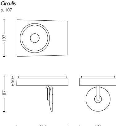
579363116 class I, IP20, SELV H50mm L273mm W197mm
