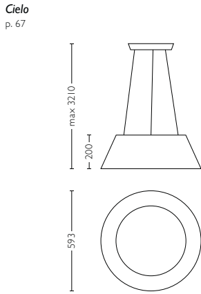
4055031LI class II, IP20, 230V H3210mm L593mm W593mm
