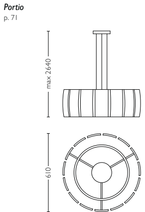
4025231LI class I, IP20, 230V H2640mm L610mm W610mm
