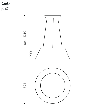
4055001LI class II, IP20, 230V H3210mm L593mm W593mm
