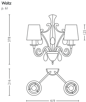
3668230LI class I, IP20, 230V H378mm L419mm W216mm
