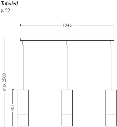
407171LI class I, IP20, SELV H2500mm L1046mm W120mm
