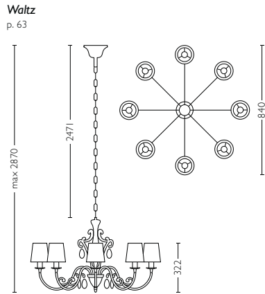
3668131LI class I, IP20, 230V H2870mm L840mm W840mm
