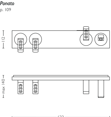
571643LI class I, IP20, SELV H140mm L622mm W112mm
