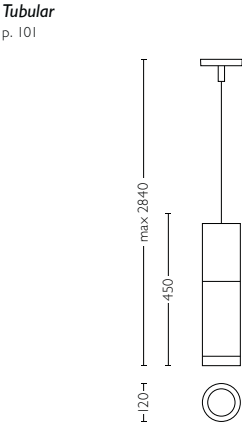
402151LI class I, IP20, 230V H2840mm L120mm W120mm
