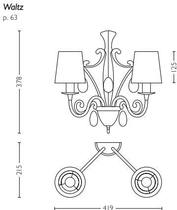
3668231LI class I, IP20, 230V H378mm L419mm W216mm
