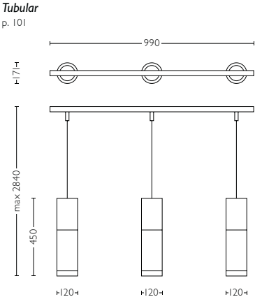
402171LI class I, IP20, 230V H2840mm L990mm W120mm
