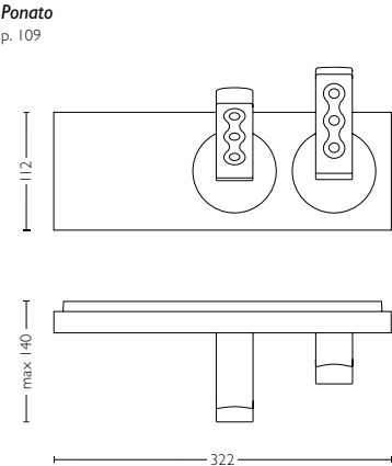
571623LI class I, IP20, SELV H140mm L322mm W112mm
